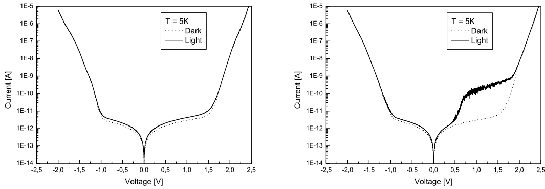
FIGURE 1. Typical behavior of dark (dotted) and photo- (solid) I-V characteristics of InAs/GaAs QDIPs at 5K.
