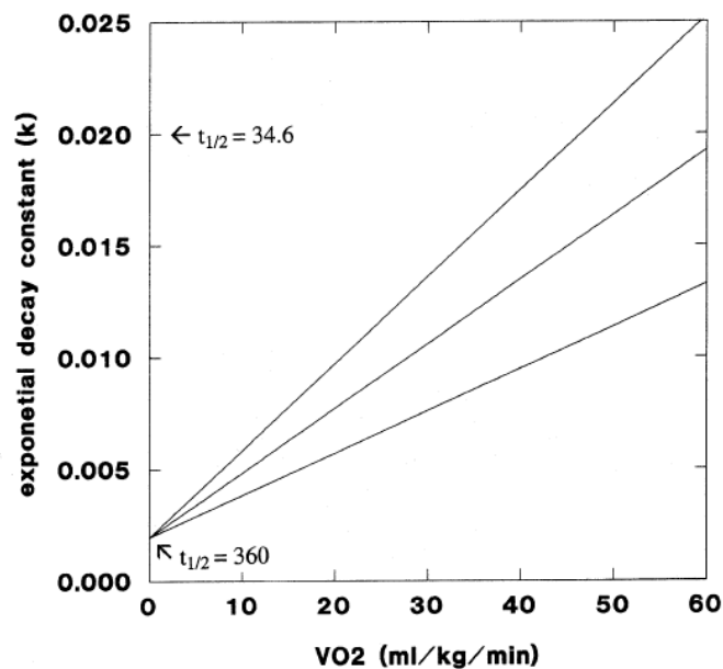
Figure 15. Linear relationship between k and VO_2 as estimated by [11]
